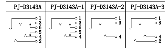
SCHEMATIC
