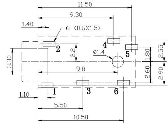
SCHEMATIC
